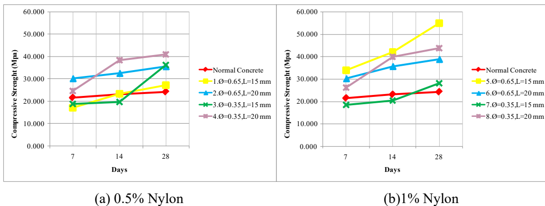
Figure 2. Compressive strength of SCC with nylon fiber.
